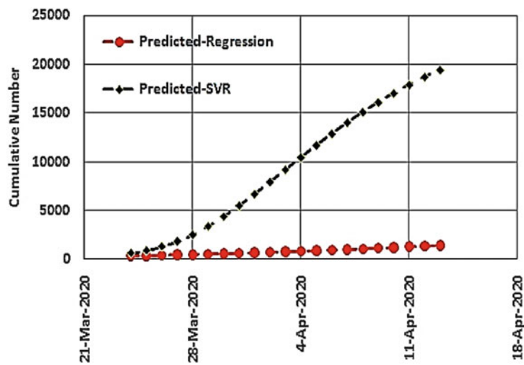
Fig. 3.16 Prediction of cumulative infection in India
