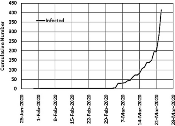
Fig. 3.19 Cumulative infection in India
