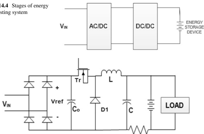
Fig. 14.5 Energy harvesting circuit: two-stage
