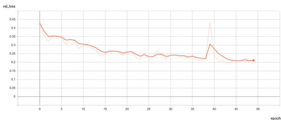
Fig. 21.16 Progression of the validation loss of InceptionV3
