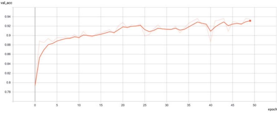
Fig. 21.11 Progression of the validation accuracy of Xception
