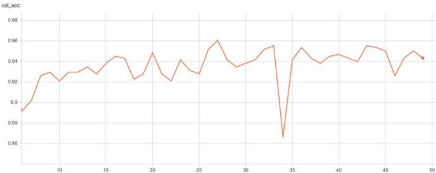
Fig. 21.5 Progression of the validation accuracy using VGG16 model
