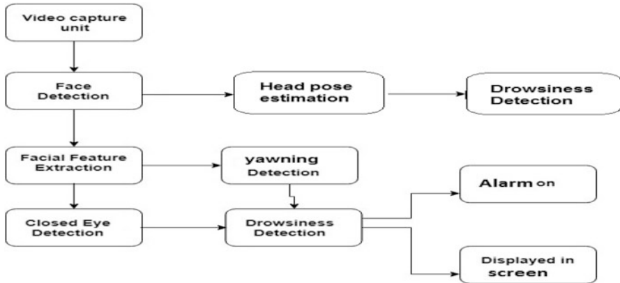
Fig. 20.10 The architecture of the proposed system
