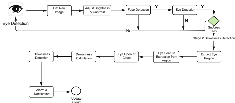
Fig. 20.9 Detailed process layout for detection of driver behaviour and drowsiness detection
