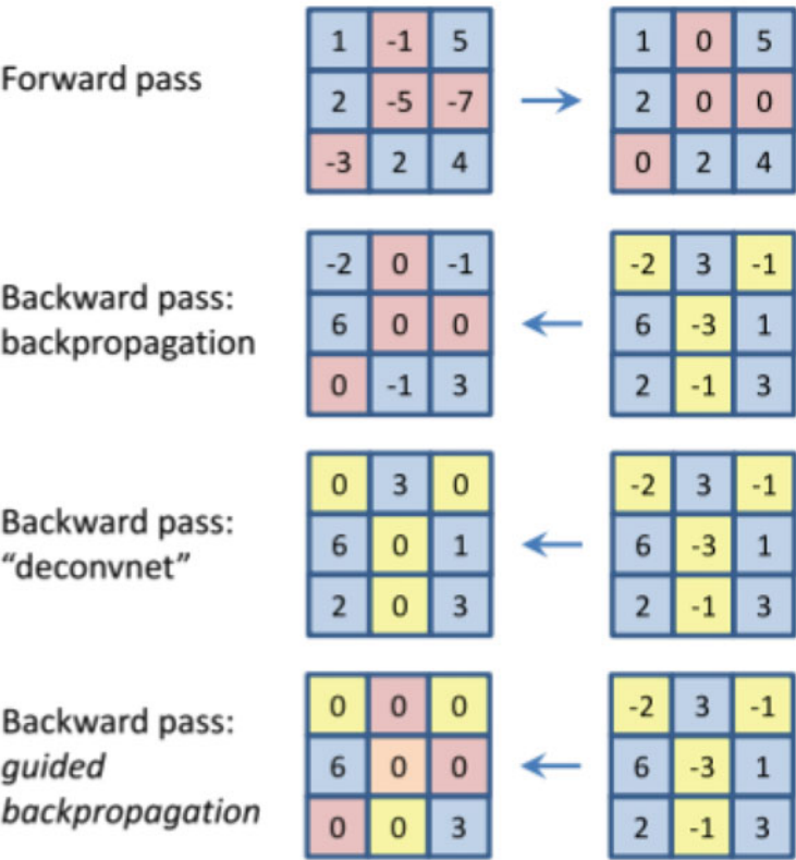
Fig. 16.2 Backpropagation methods [16]
