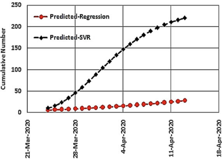
Fig. 3.22 Estimation of cumulative death in India
