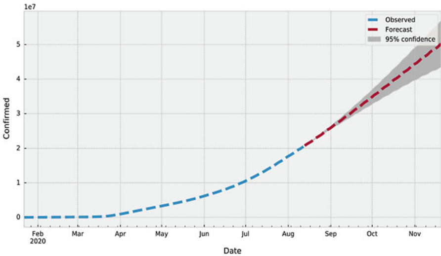
Fig. 8.15 ARIMA forecast
