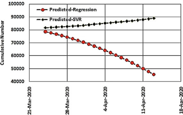
Fig. 3.14 Prediction of cumulative infection in China
