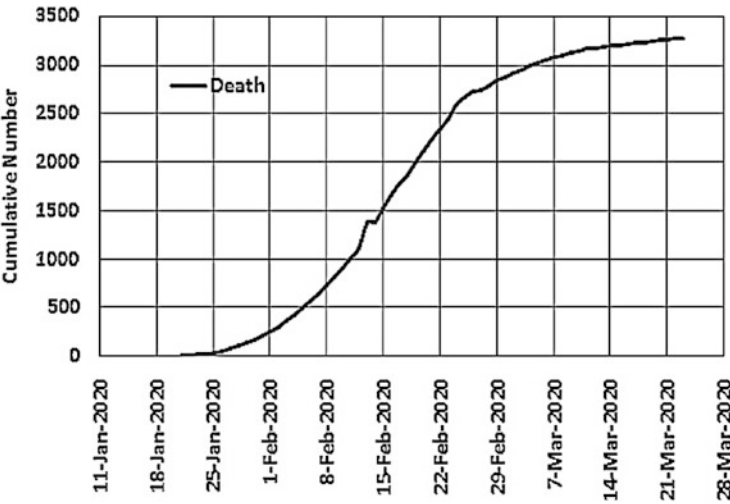
Fig. 3.23 Cumulative death in China
