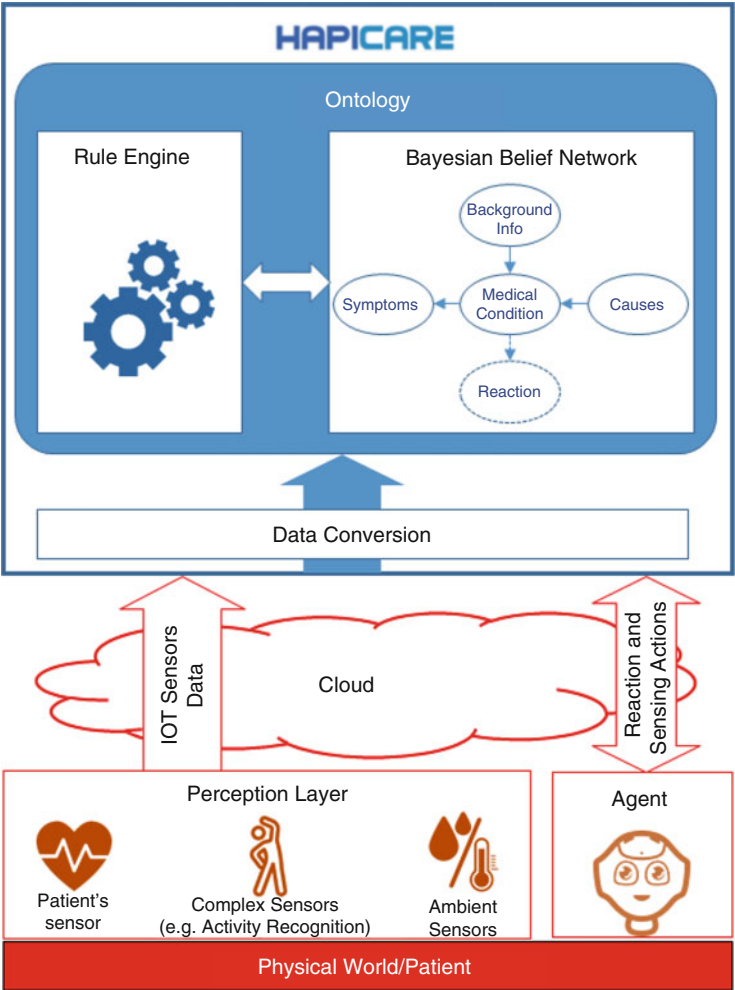
Fig. 2.2 Overview of the Maidis Hapicare platform architecture
