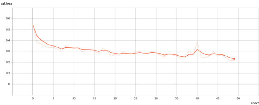
Fig. 21.12 Progression of the validation loss of Xception
