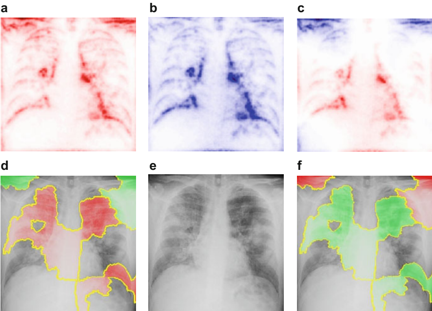
Fig. 16.7 LRP-PresetAflat and LIME explanation for each class for a Covid-19 image. (a) LRP-Covid. (b) LRP-Normal. (c) LRP-Viral. (d) LIME-Covid. (e) LIME-Normal. (f) LIME-Viral
