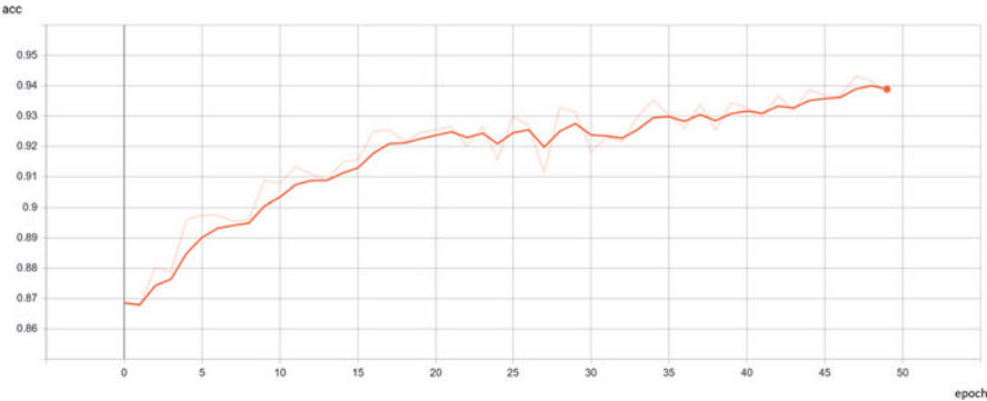
Fig. 21.9 Progression of the training accuracy of Xception
